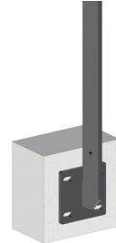
F4 - Face Mount (4 Fixings)
