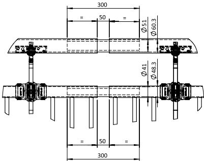
EXPANSION JOINT DETAILS DETAIL A SCALE 1 : 10
