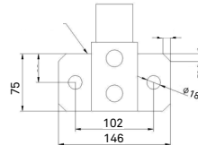
F2 - Face Mount (2 Fixings)
