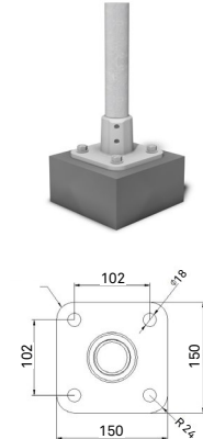
T4 - Top Mount (4 Fixings)
